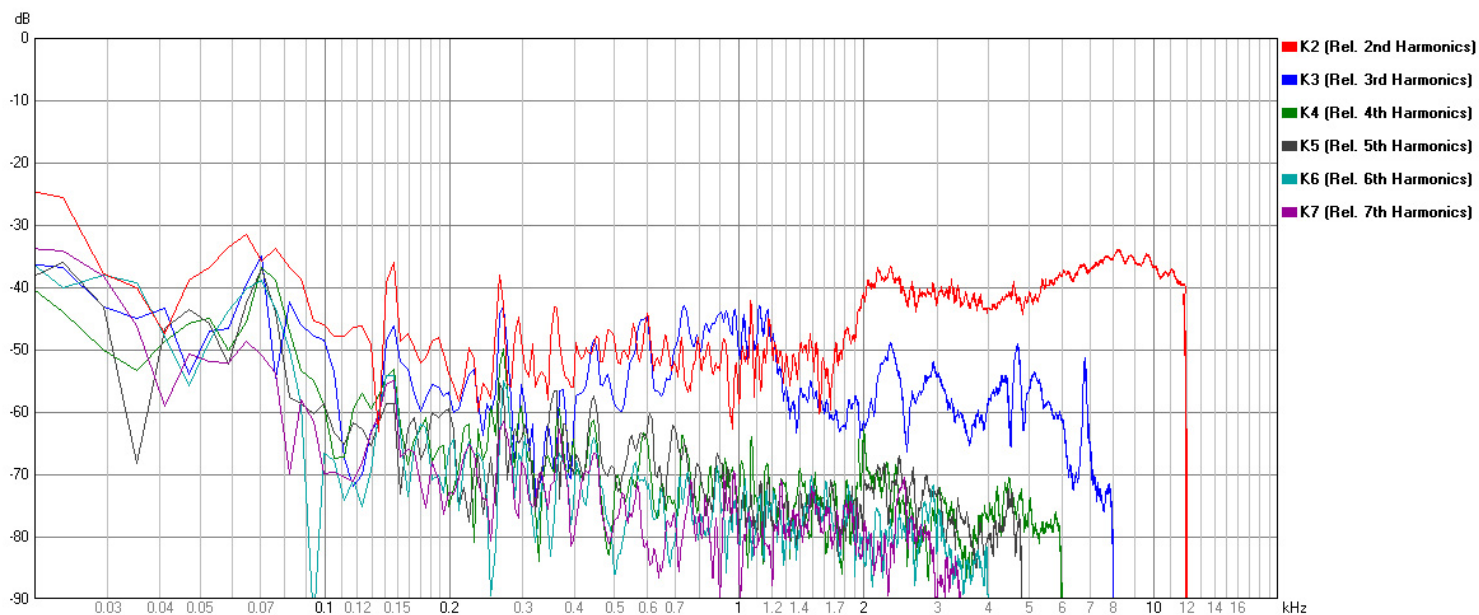
Air Motion mk2 2nd - 7th relative harmonics
